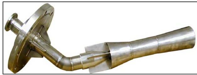
Hastelloy Jet Mixer on Tank support
